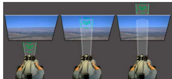
Figure 7. Appearance Of HMD Symbolry Relative To OTW Imagery As The Viewer Electronically Adjusted Vergence Settings On The HMD
